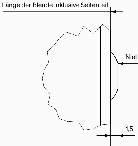
DETAIL X
