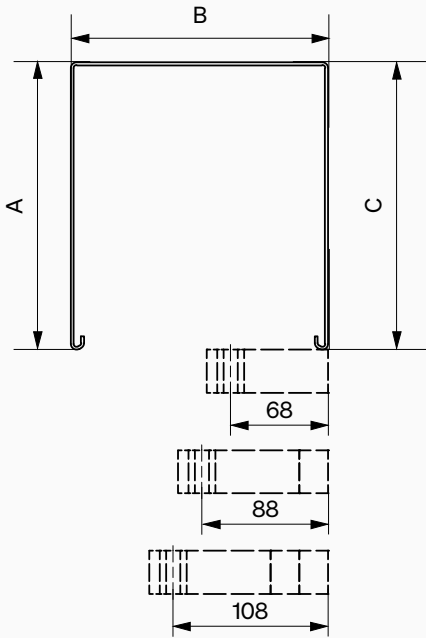
Lambrequins sans pliage D (F11, F21, F30, F33)
