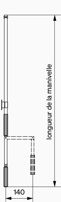
Manivelle standard
